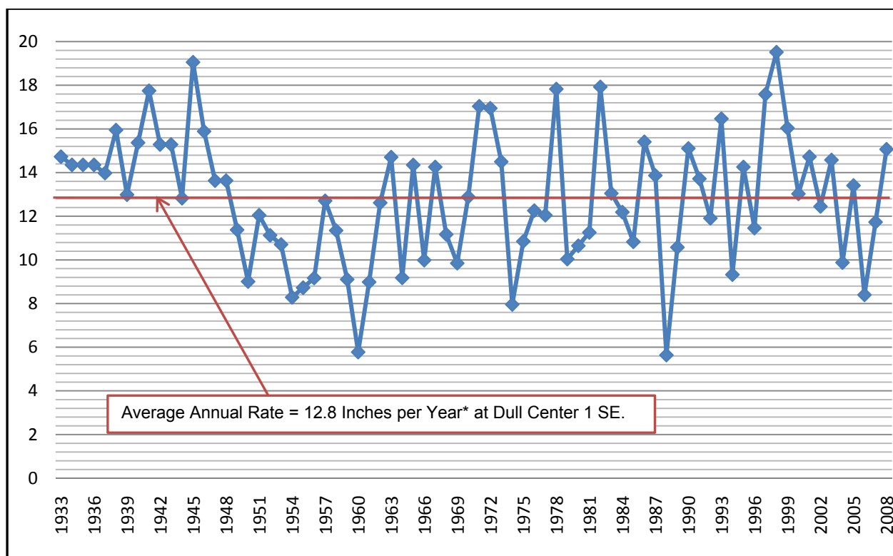
Figure 2.1.2-1 Precipitation for Dull Center, Wyoming in inches per year.
