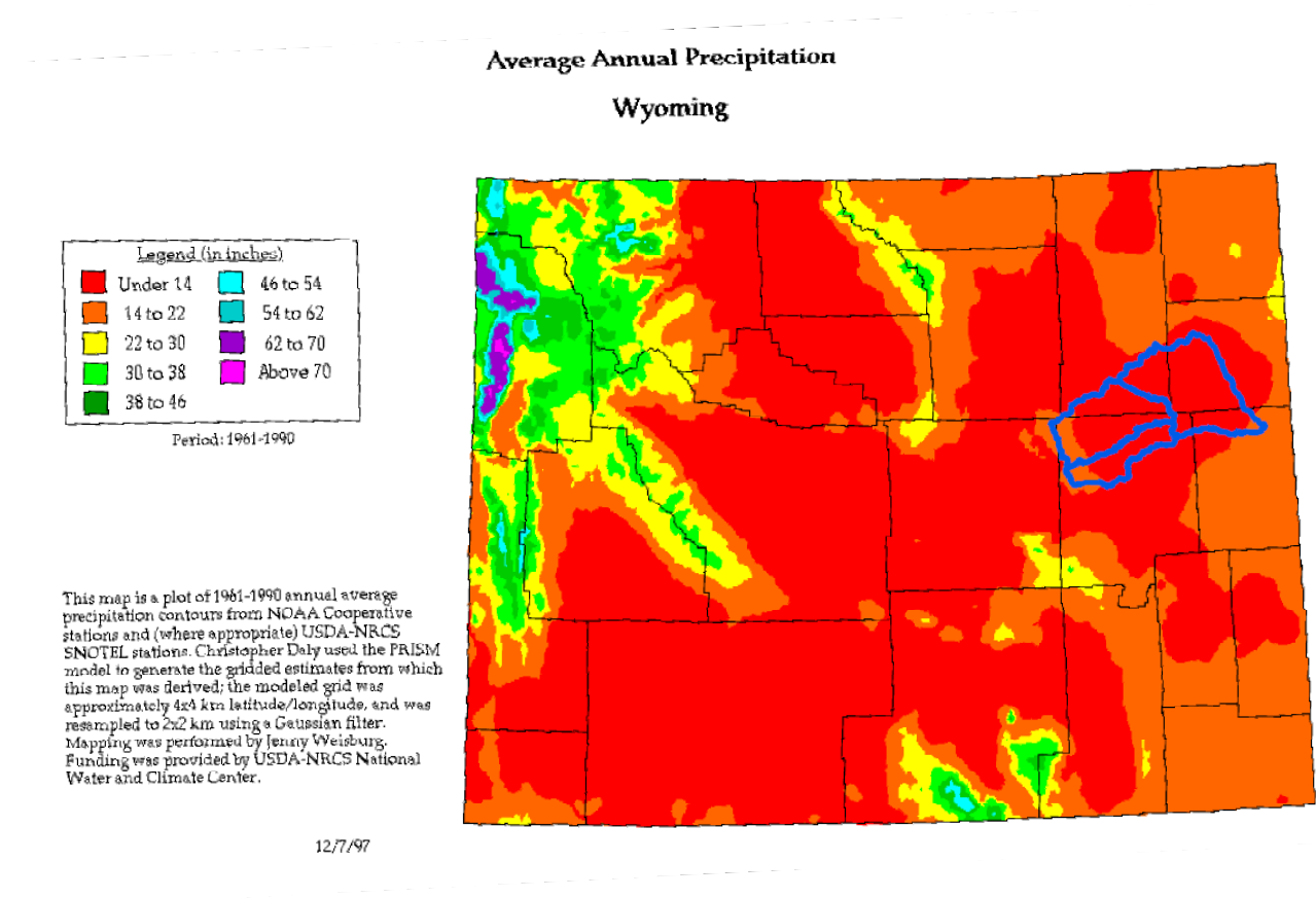
Figure 2.1.2-2 Average Annual Precipitation of Wyoming with Thunder Basin Watershed and the three subbasins in blue.
